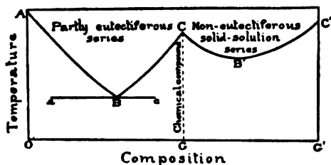
Fig. 53. Supposititious Freezing-point Curve of a Series Containing a Definite Chemical Compound and Eutectiferous at One End but not at the Other.
